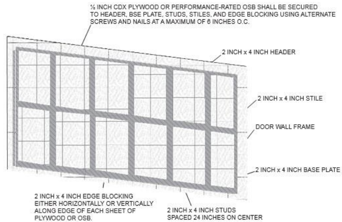
FIGURE A103.1(2) BOARDING OF DOOR WALL
