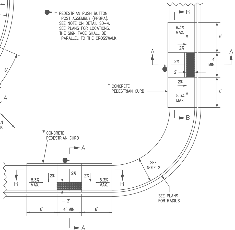
CURB RAMP TYPE 2B
