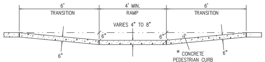
SECTION B-B
