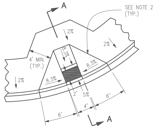
RAMP DETAIL
