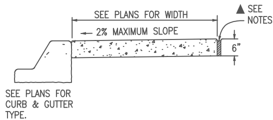
CONCRETE SIDEWALK
